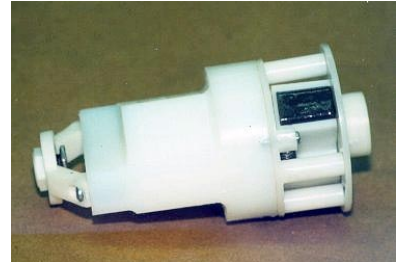
Extended Cutter Head for longer than standard strip length.
